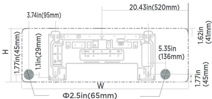
Indoor unit dimensions(WxH): 38.2in(971mm)x12.6in(321mm)
